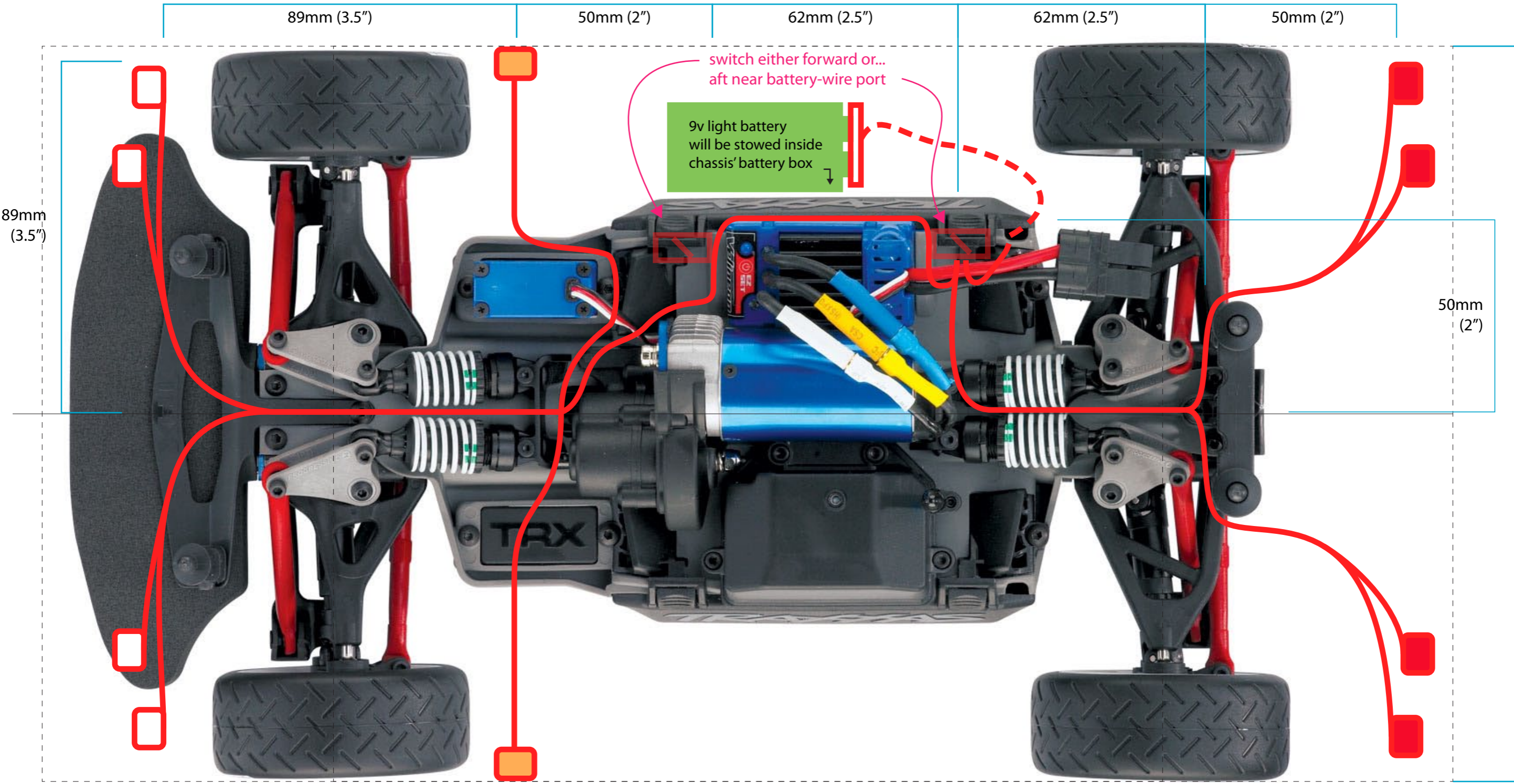
Traxxas Rally VXL 1/16 10-LED chassis lighting rig Ryan Hicks [//] Prototyp
